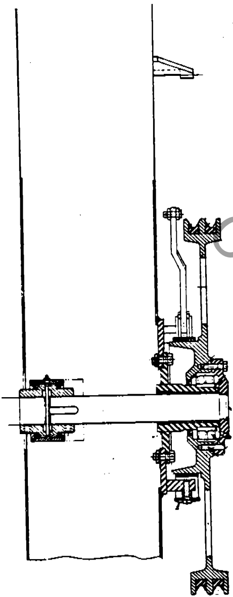
HOLDING BRAKE (OLDER UNITS)
