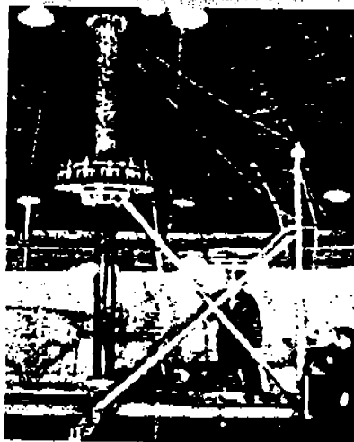
3. Center pole is erect. Lower end of brace leg is about to be planned to mud sill. Note that winch pole is braced by two of the four brace legs of center pole. Later these brace legs will be detached from winch pole and placed in their own positions as braces for center pole.
