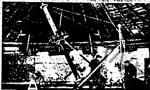
2. Up she goes! With less tension on winch, one man can now operate it and brake at same time. Other man guides brace leg to pin slot on mud sill.
