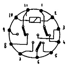
INSIDE HELE' (R1 R2) ELECTRICAL CONNECTIONS
